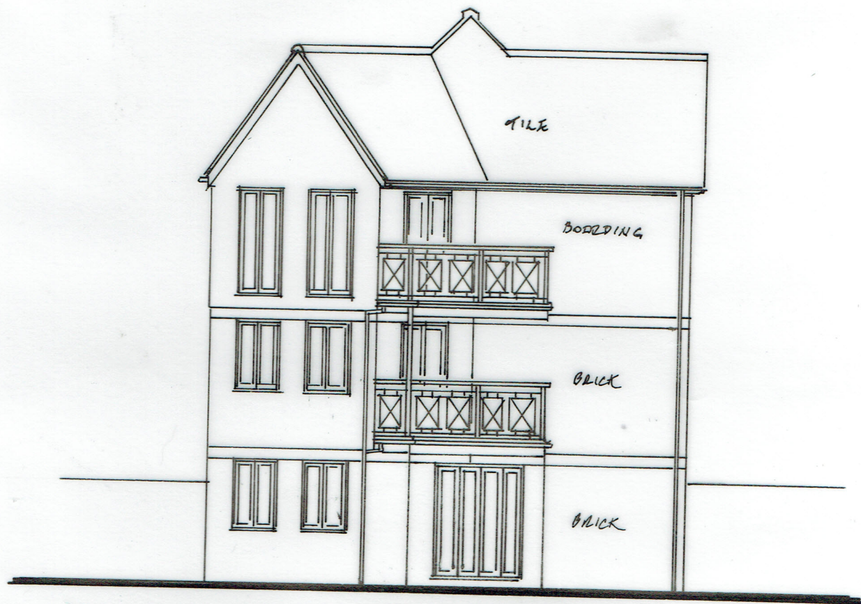
EXISTING NORTH EAST ELEVATION (REAR)
